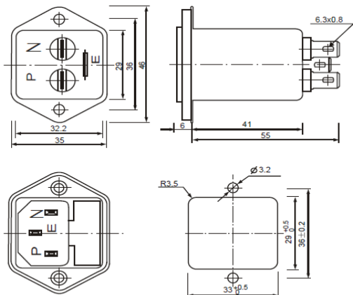
Panel Cut Out fig. 1
