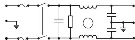
fig.3 (for two fuses)
