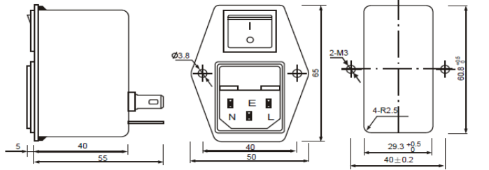
fig. 2 Panel Cut Out
