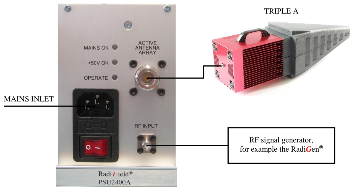
Figure 2: Overview of the RadiField® plug-in card connections
