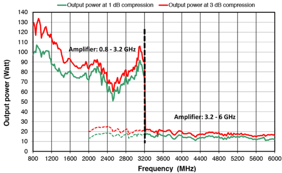
SX70/15 POWER AMPLIFIER 70W-15W / 800 MHz - 6000 MHz
