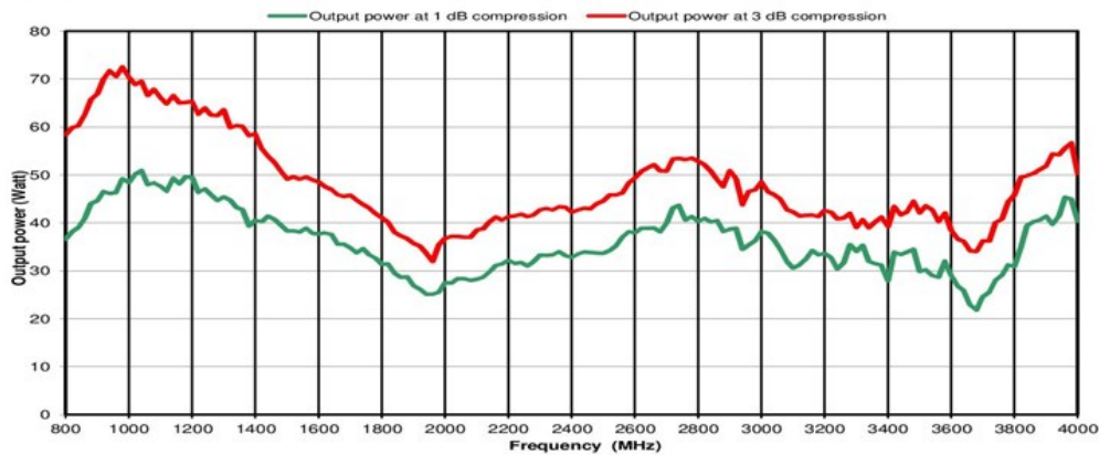
SW35 POWER AMPLIFIER 35W / 800 MHz - 4 GHz
