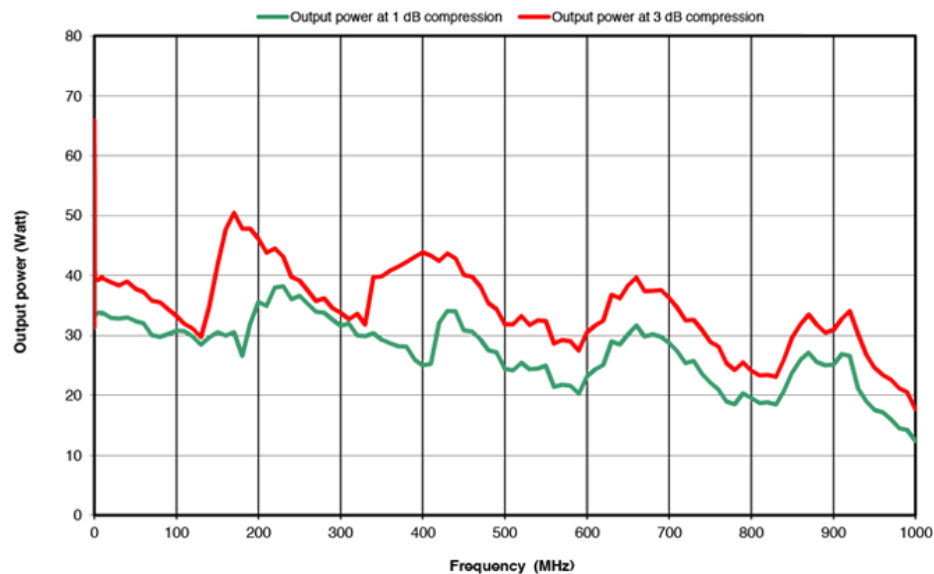
DT25 POWER AMPLIFIER 25W / 10 kHz - 1000 MHz
