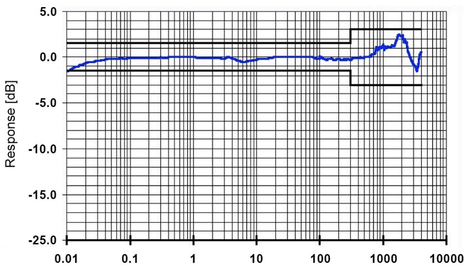
RSS1004A Typical frequency response with limits.
