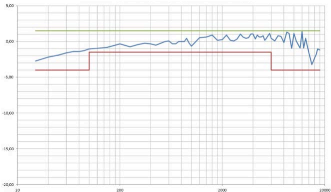
RSS1018A Typical frequency response with limits (dB).
